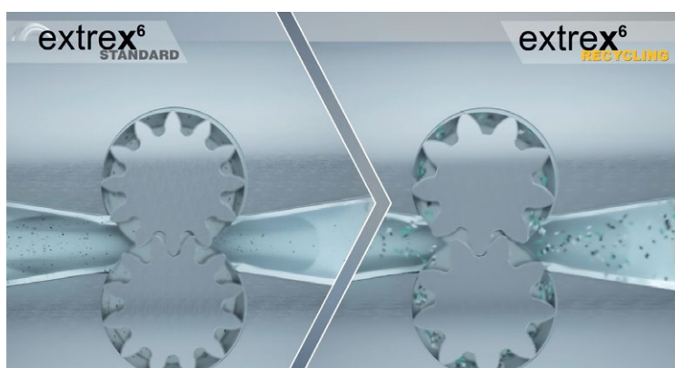
Comparison of extrex6 standard pump and extrex6 recycling pump: MAAG's melt pump has been specially upgraded for processes dealing with higher contamination levels and larger particles on the recycling market
