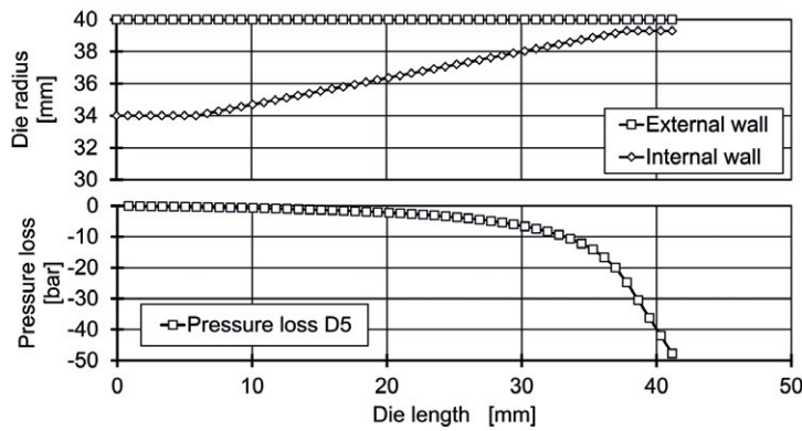
Fig. 5: Influence of die design D5 ( D_g = 0.7 mm, L_{pa} = 4 mm, \angle = 80^\circ ) on pressure loss
